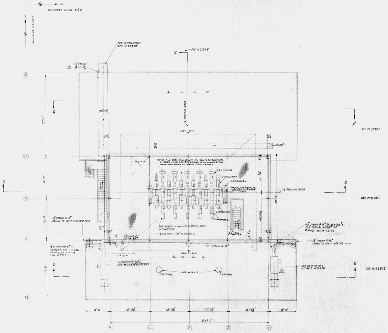
PLAN - EL. +80'-5 1/2"
